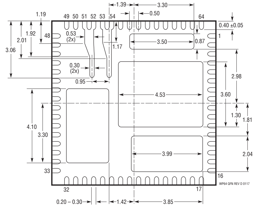
BOTTOM VIEW (BOTTOM METALLIZATION DETAILS)
